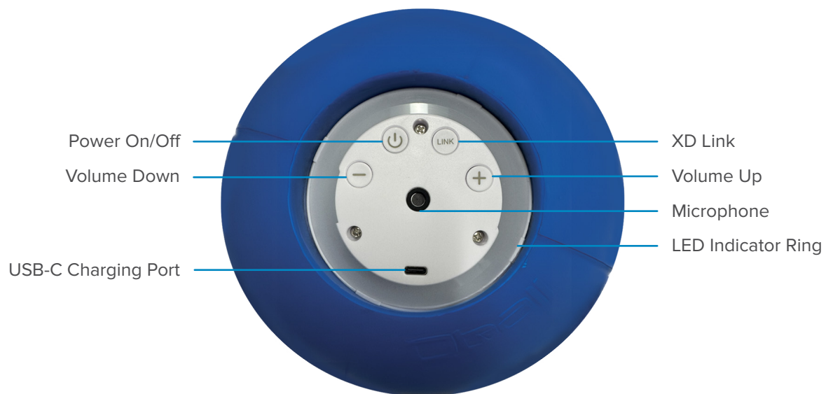
Top View Without Cover
